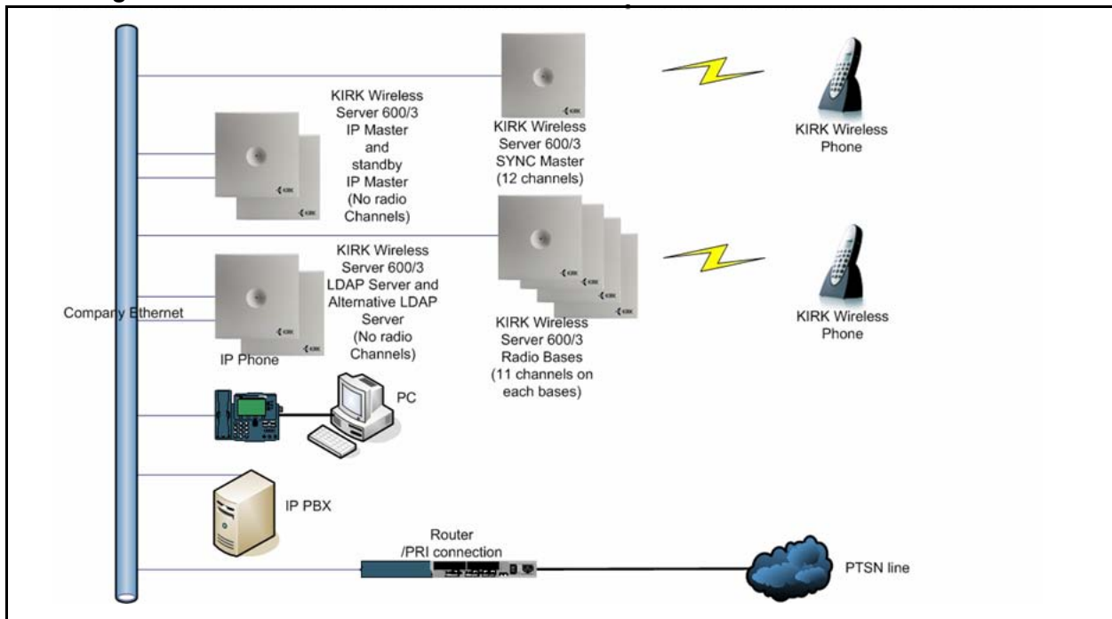
Figure 80 KWS600v3 Multi-cell installation with Alternative LDAP Server
